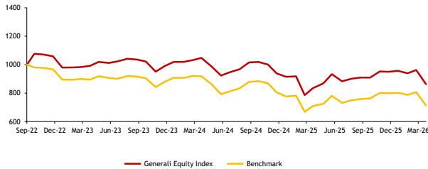
Generali Equity Index vs Tolak Ukur
